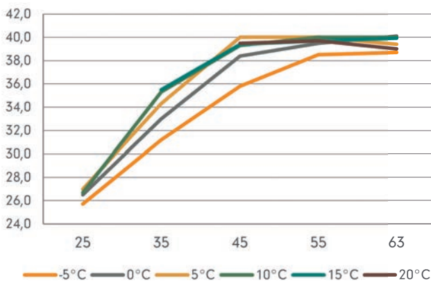
Max external pressure loss, Brine [kPa - l/s]
