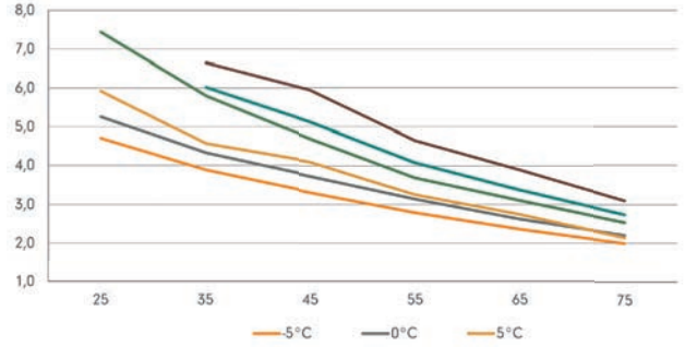
Max external pressure loss, Charge [kPa - l/s]
