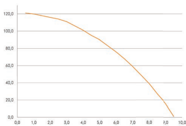
Max external pressure loss, Charge [kPa - l/s]
